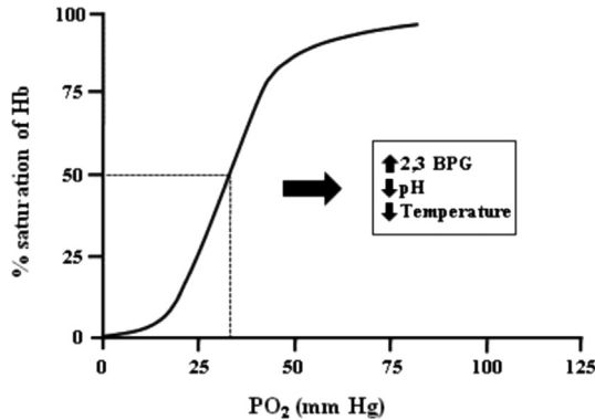
Fig. 2. The oxyhemoglobin dissociation curve representing the nonlinear relationship between PO_2 and oxygen saturation ( SpO_2 ). The curve shifts to the right in response to increased 2,3-BPG concentration within the RBC, severe acidemia, and hypothermia. The dashed line indicates the partial pressure of oxygen at which Hb is 50% saturated under physiologic conditions ( P_{50} ).
